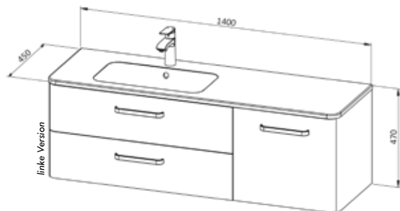
CHARM 140 , 1 Tür, 2 Schubladen L/R ● ●
