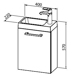
ARWEN SMALL 40, 1 Tür, L/R
